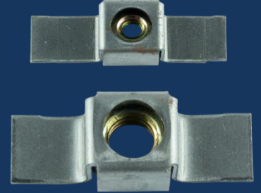
3/16" to 5/16" BSW/UNC
